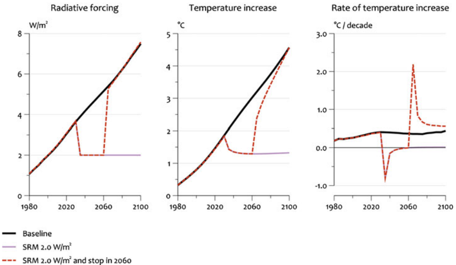
Fig. 4 Radiative forcing ( left ), global mean temperature increase above pre-industrial levels ( middle ), and rate of temperature change ( right panel) in the SRM-scenario, including a variant in which SRM is ceased in 2060 (SRM = Solar Radiation Management)
