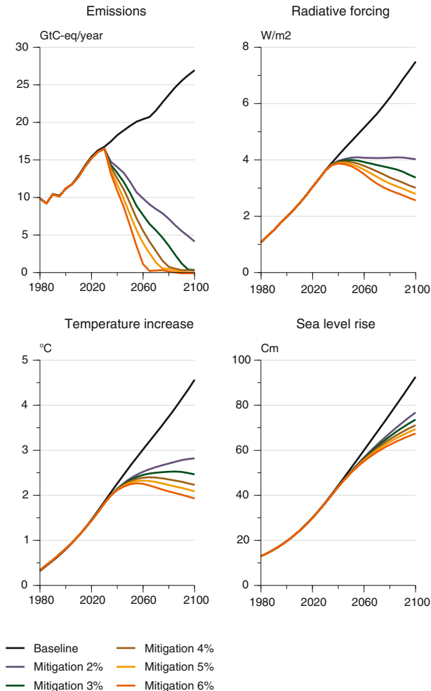
Fig. 5 Greenhouse gas emissions, radiative forcing, global mean temperature increase above pre-industrial levels and sea level rise: sensitivity runs exploring reduction rates of energy/process-related CO 2 of 2–6 % (assuming a floor of –2 GtC/per year). Other emissions have been coupled on the basis of correlation in existing scenarios, except for CO 2 emissions from land-use for which the results of the mitigation scenario presented in Fig. 3 has been used
